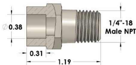
954A-06-04 3/8" Tube X 1/4" Male NPT
