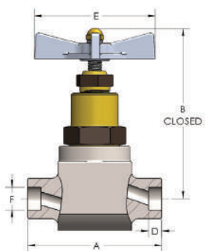
370 - Welded Globe
