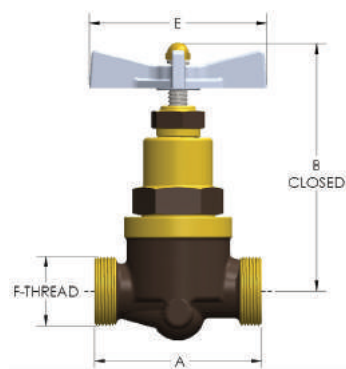
380 - Globe
