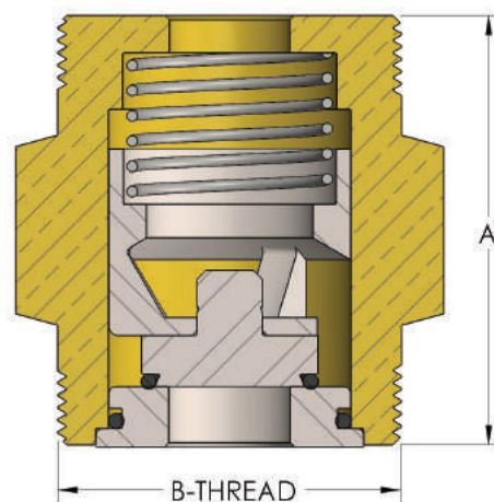
123A - In-line
