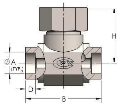
Globe Check Valve
