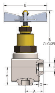
371 - Welded Angle
