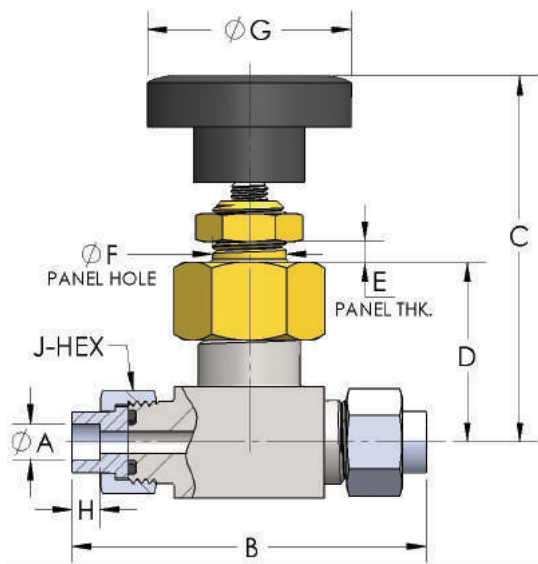
Inline
