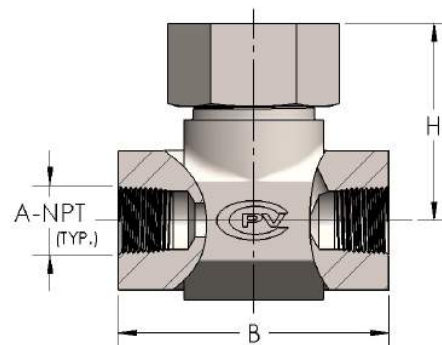
Globe Check Valve
