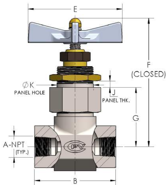
Globe Hand Valve
