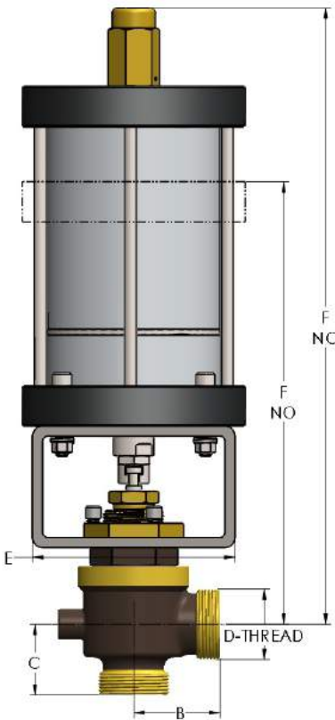
1381 Valve
