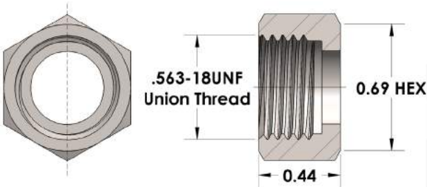
950N-04 Standard Union Nut
