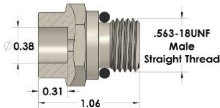
959A-06-06 3/8" Tube X Male Straight Thread
