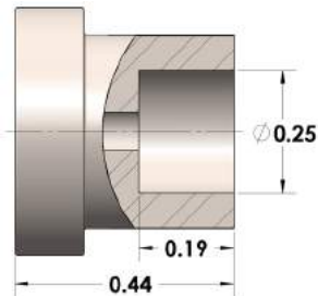
949R-04 Standard Tailpiece for 1/4" Socketweld Tube
