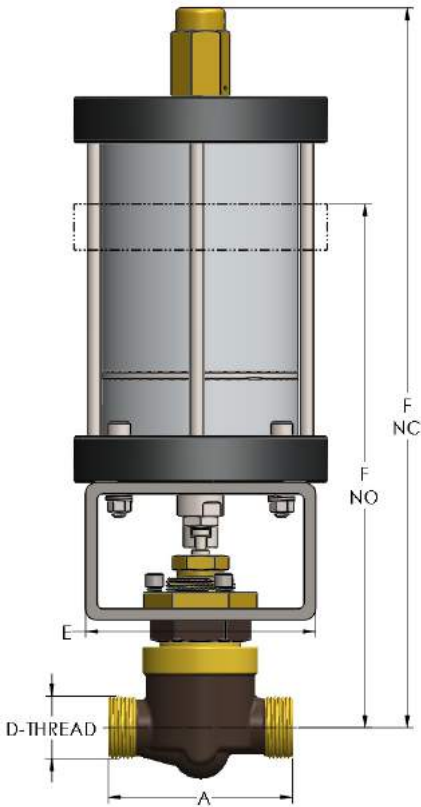
1380 Valve
